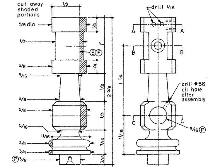
1 3/8 COLUMN Steel 3/16
