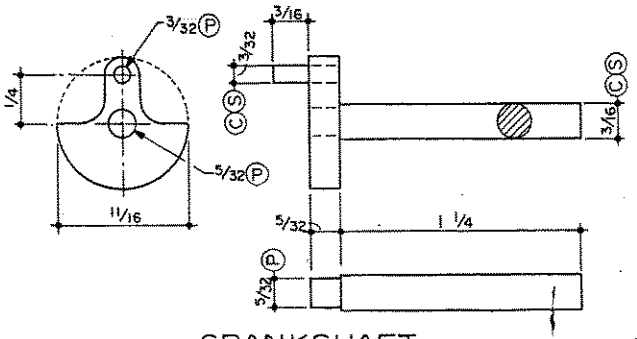
CRANKSHAFT Steel
