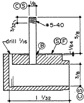
CYLINDER Brass
