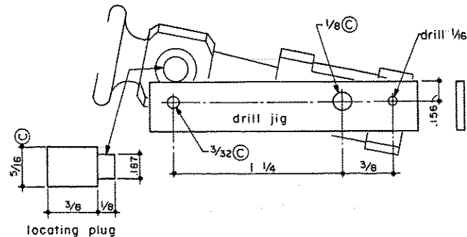
locating plug
